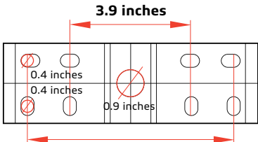
B-b. STLSTC-TRR-20W/30W (for SUNLIKE 20W/30W) works with 2.0 inches to 4.7 inches poles.
