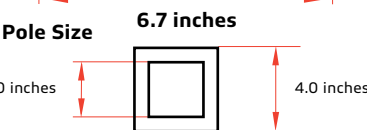
C-b. STLSTC-TRS-20W/30W (for SUNLIKE 20W/30W) works with 2.0 inches to 4.0 inches poles.
