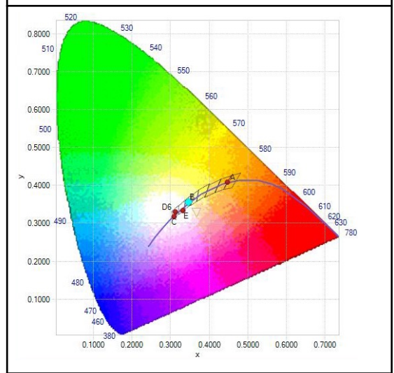
CIE LUV BINNING CURVE LIN-140 CIE 1932 – 2 Degree
