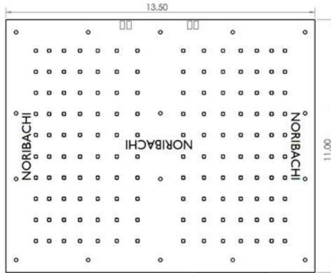
CLU-SQUARE: 140 LEDs
