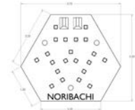
CLU-HEX: 21 LEDs
