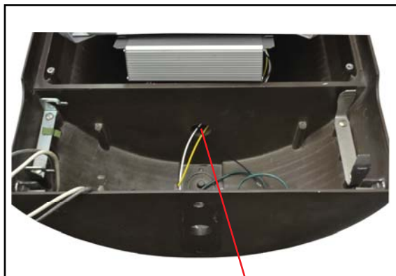
Pull ballast leads through
